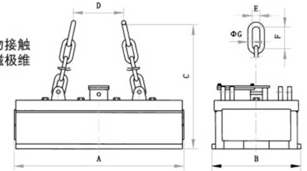
外形尺寸图 Overall Dimension Drawing
