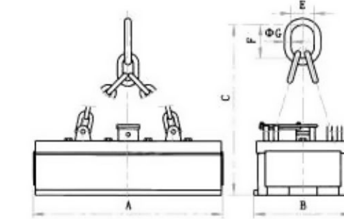
单挂点B型：单挂点与行车主钩或挂梁联接 Single Suspending Point Mode B I: the single suspending point is jointed with crane hook or suspension beam
