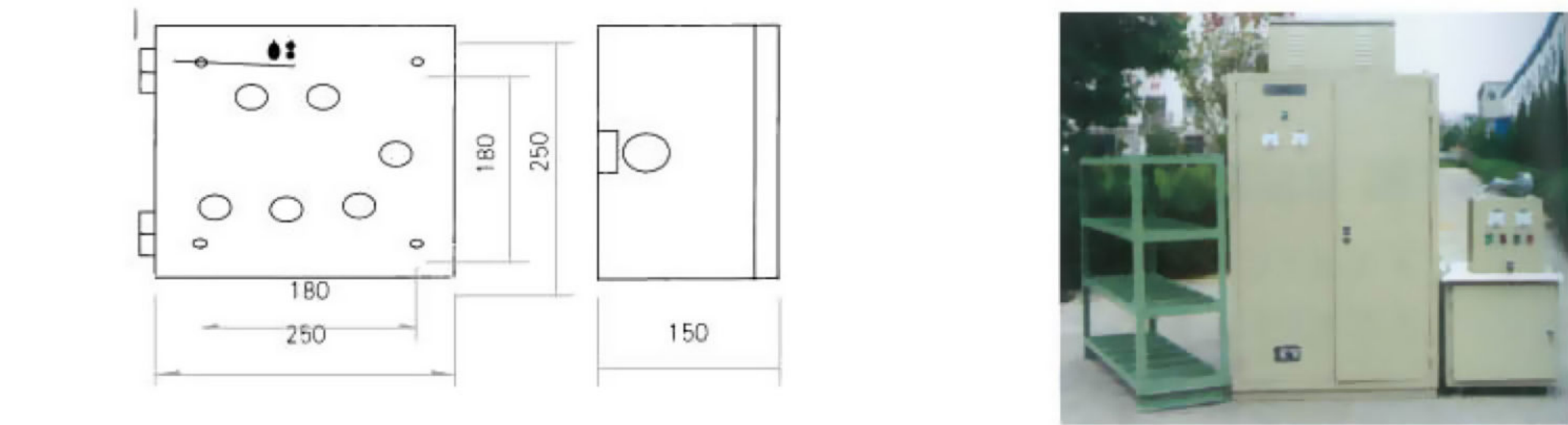
外形尺寸图 控制柜、变压器、同STQL系列操作盒外形尺寸图。 Appearance dimensions drawings of the control cabinet, transformer are same with the Manipulation box of STQL series.
