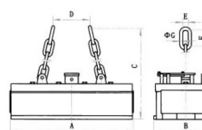
双挂点C I型：双挂点与行车主钩或挂梁联接 Double Suspending Point Mode C I: the double suspending points are jointed with crane hook or suspension beam
