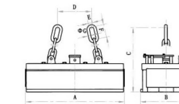
双挂点C II型：双挂点与行车主钩或挂梁联接 Double Suspending Point Mode C II: the double suspending points are jointed with crane hook or suspension beam
