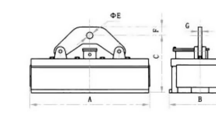
单挂点B II型：单挂点与行车主钩或挂梁联接 Single Suspending Point Mode B II: the single suspending point is jointed with crane hook or suspension beam
