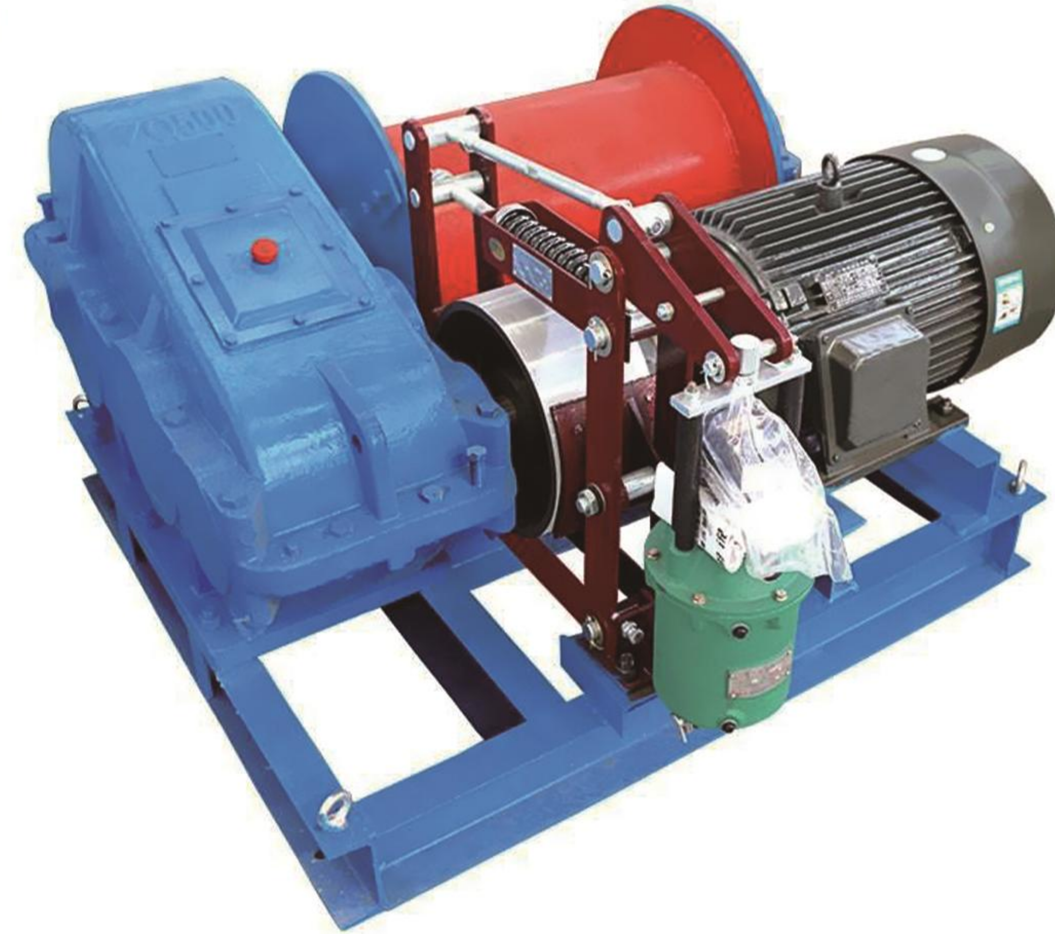
JM Type electric winch
