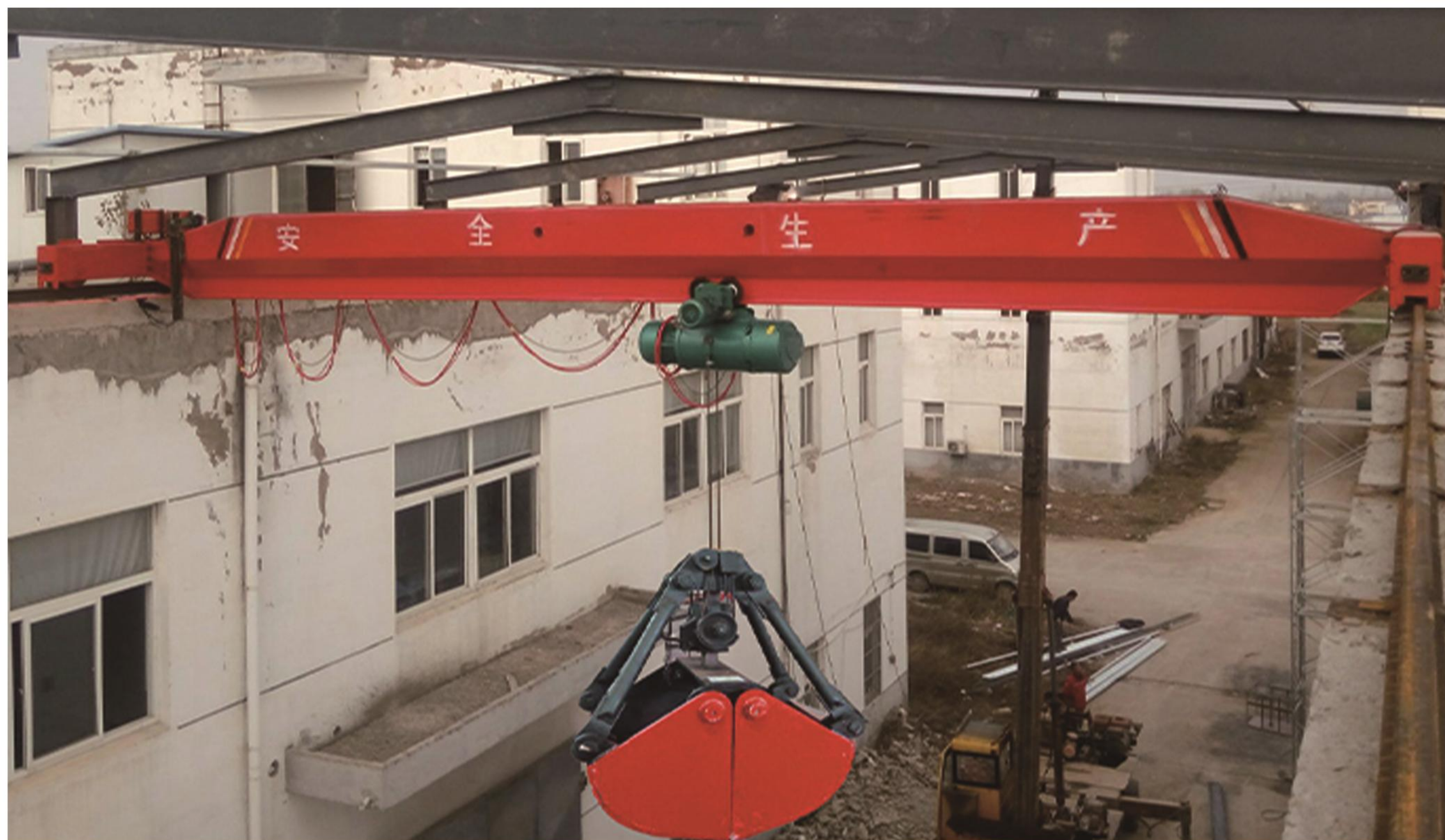
LDZ Type single beam grab overhead crane
