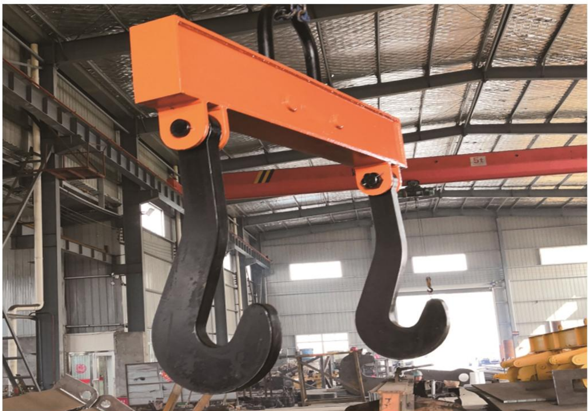
Ladle hook
